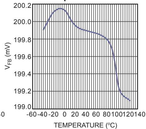
V_{FB} Regulation Voltage vs. Temperature
