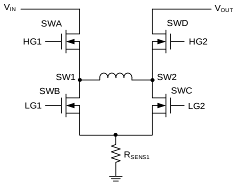
Figure 3: Buck-Boost Topology
