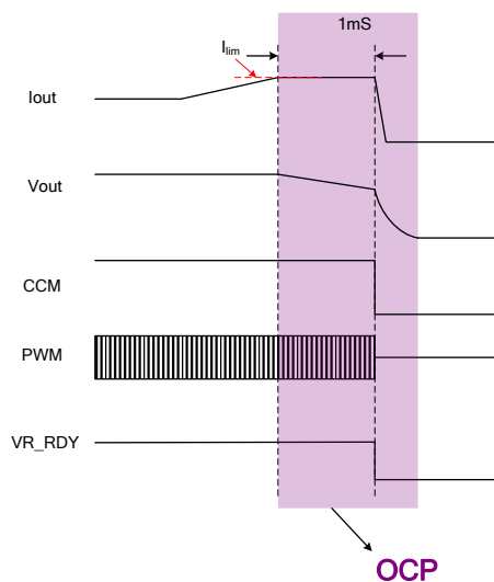
Figure 12: OCP Fault Protection
