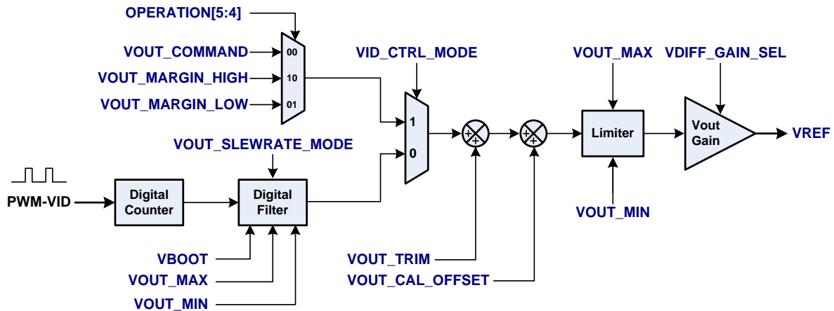
Figure 20: Conceptual View of how Output Voltage Related Commands are Applied
