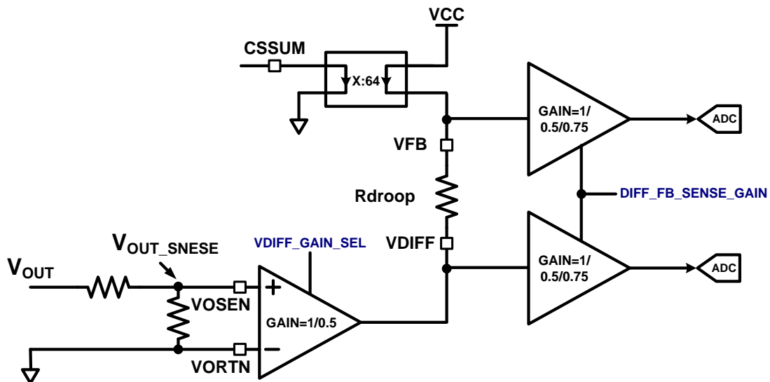
Figure 18: DC Loop Gain Selection Block Diagram
