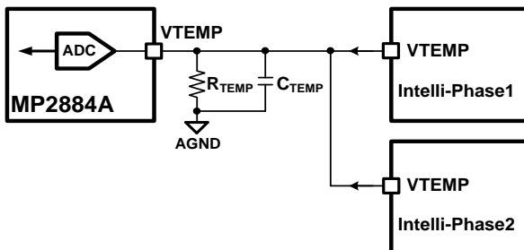
Figure 9: Temperature Sense with Intelli-Phase
