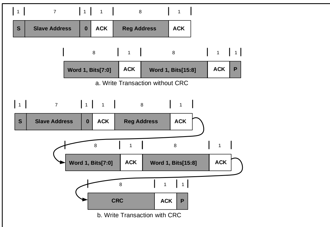
Figure 19: I²C Write Transaction
