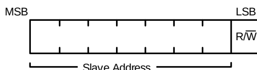
Figure 16: 7-Bit Address
