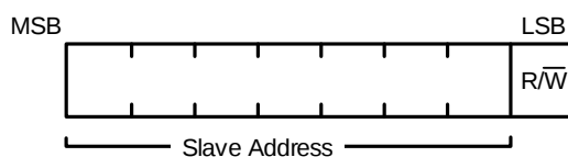
Figure 12: 7-Bit Addressing
