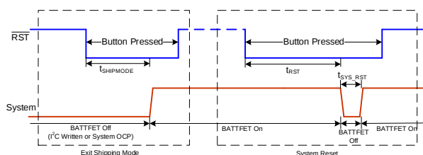
Figure 6: RST Timing
