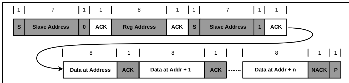
Figure 14: Multi-Read Sequence
