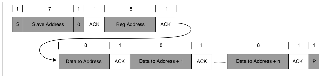
Figure 12: Multi-Write
