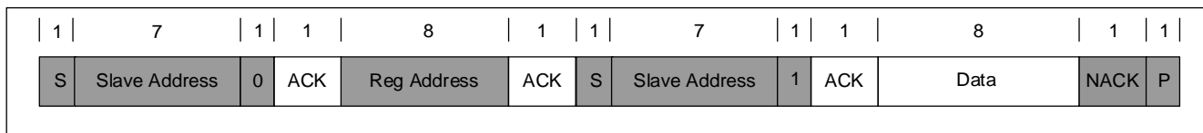
Figure 11: Single-Read
