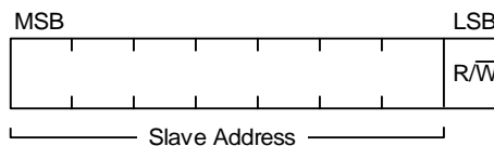
Figure 8: 7-Bit Address
