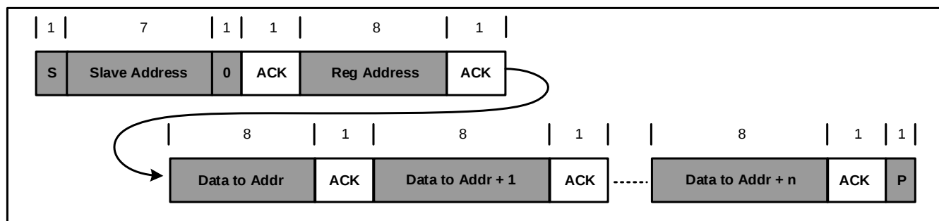
Figure 14: Multi-Write
