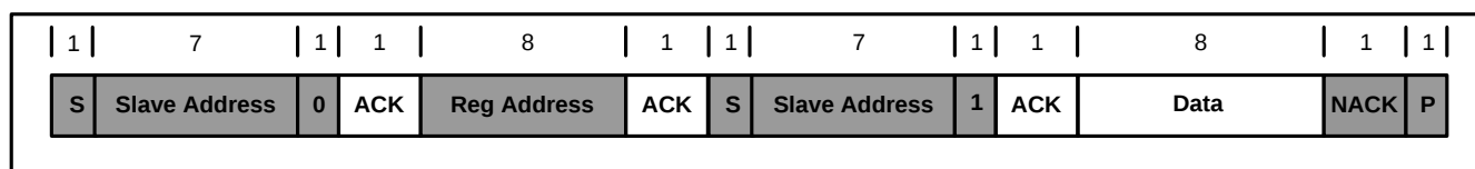
Figure 13: Single Read
