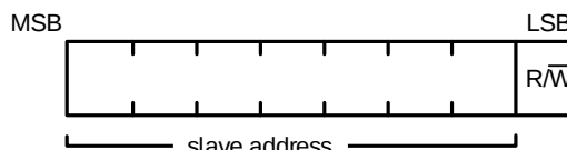
Figure 10: 7-Bit Address
