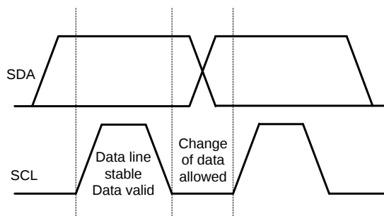
Figure 9: Bit Transfer on the I 2 C Bus
