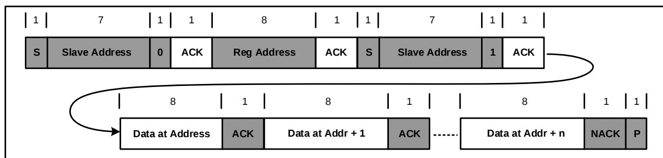
Figure 15: Multi-Read
