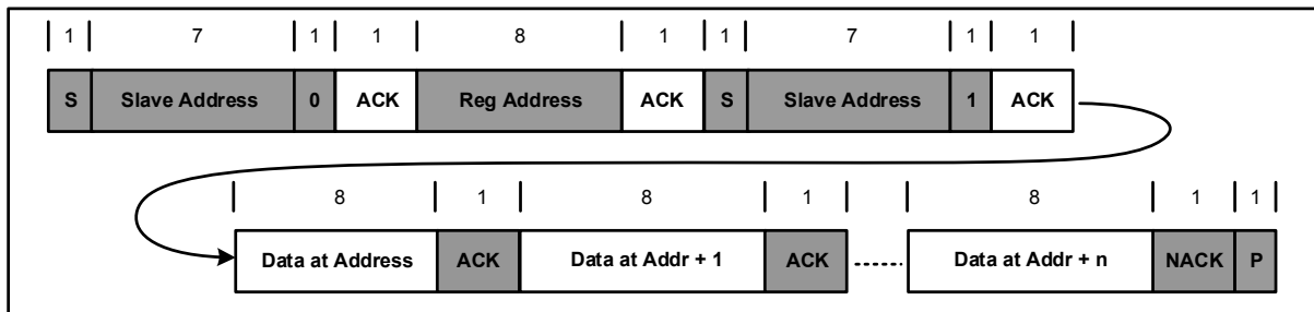
Figure 15: Multi-Read
