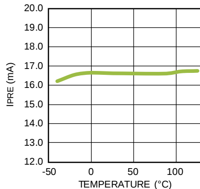
Pre-Charge Current vs. Temperature
