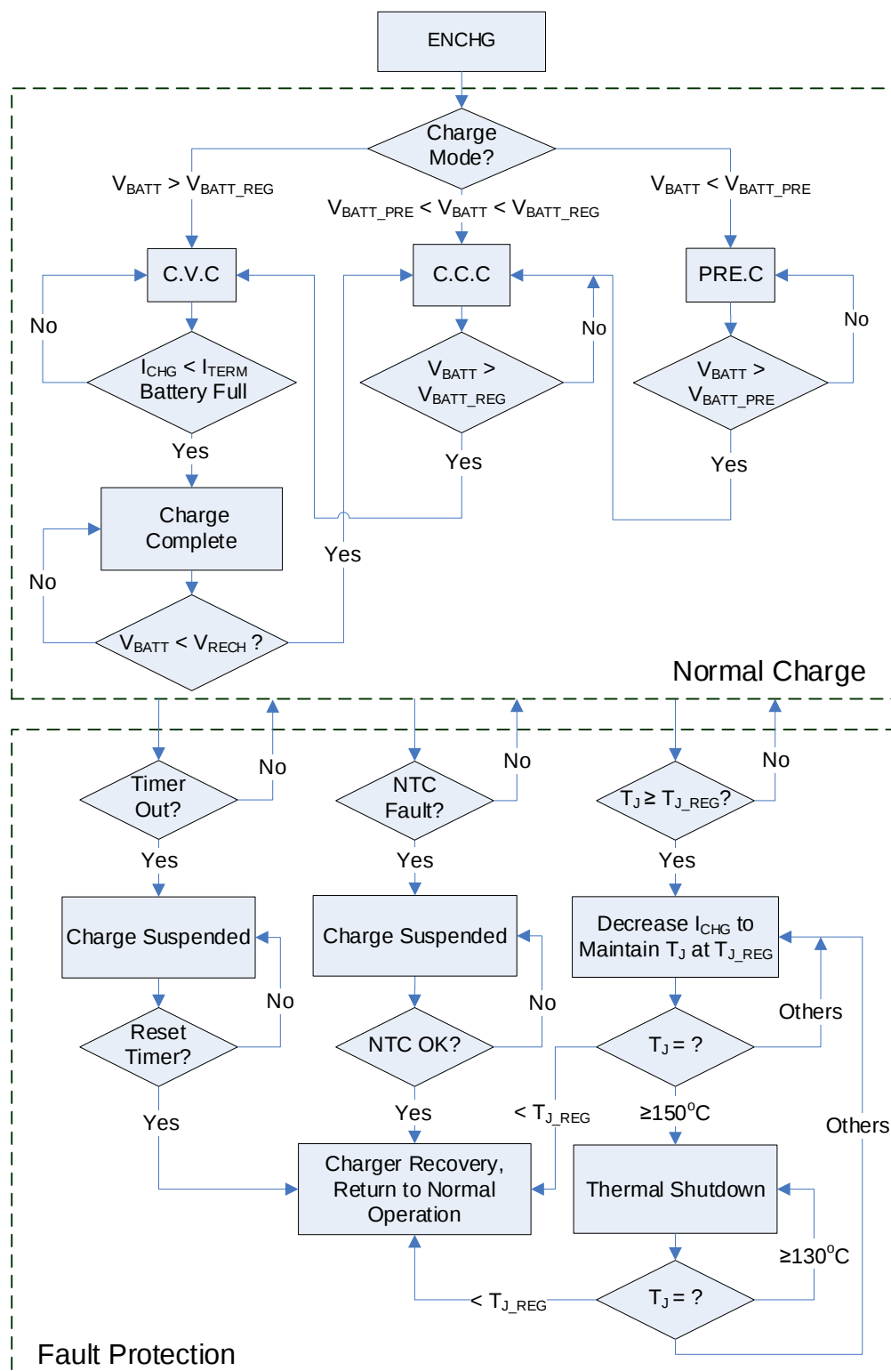
Figure 18: Charging Process
