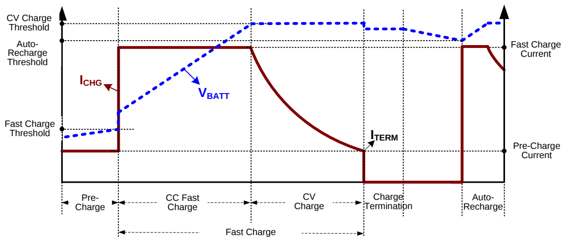
Figure 4: Battery Charge Profile
