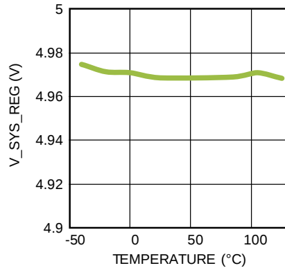
System Regulation Voltage vs. Temperature
