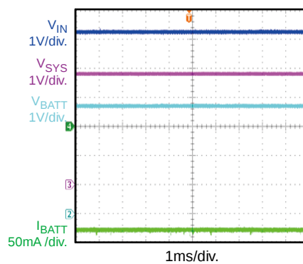
Input Current Limit based PPM
