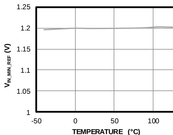
VIN_MIN Voltage Reference vs. Temperature
