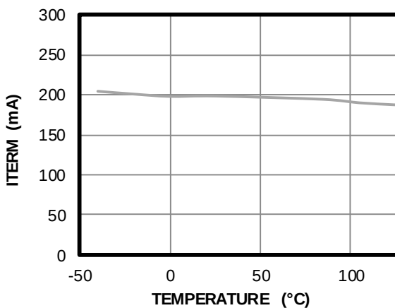
Termination Current vs. Temperature
