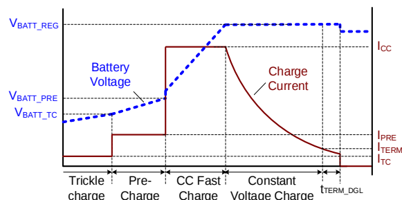
Figure 3: Battery Charging Cycle
