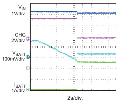
Auto Recharge
