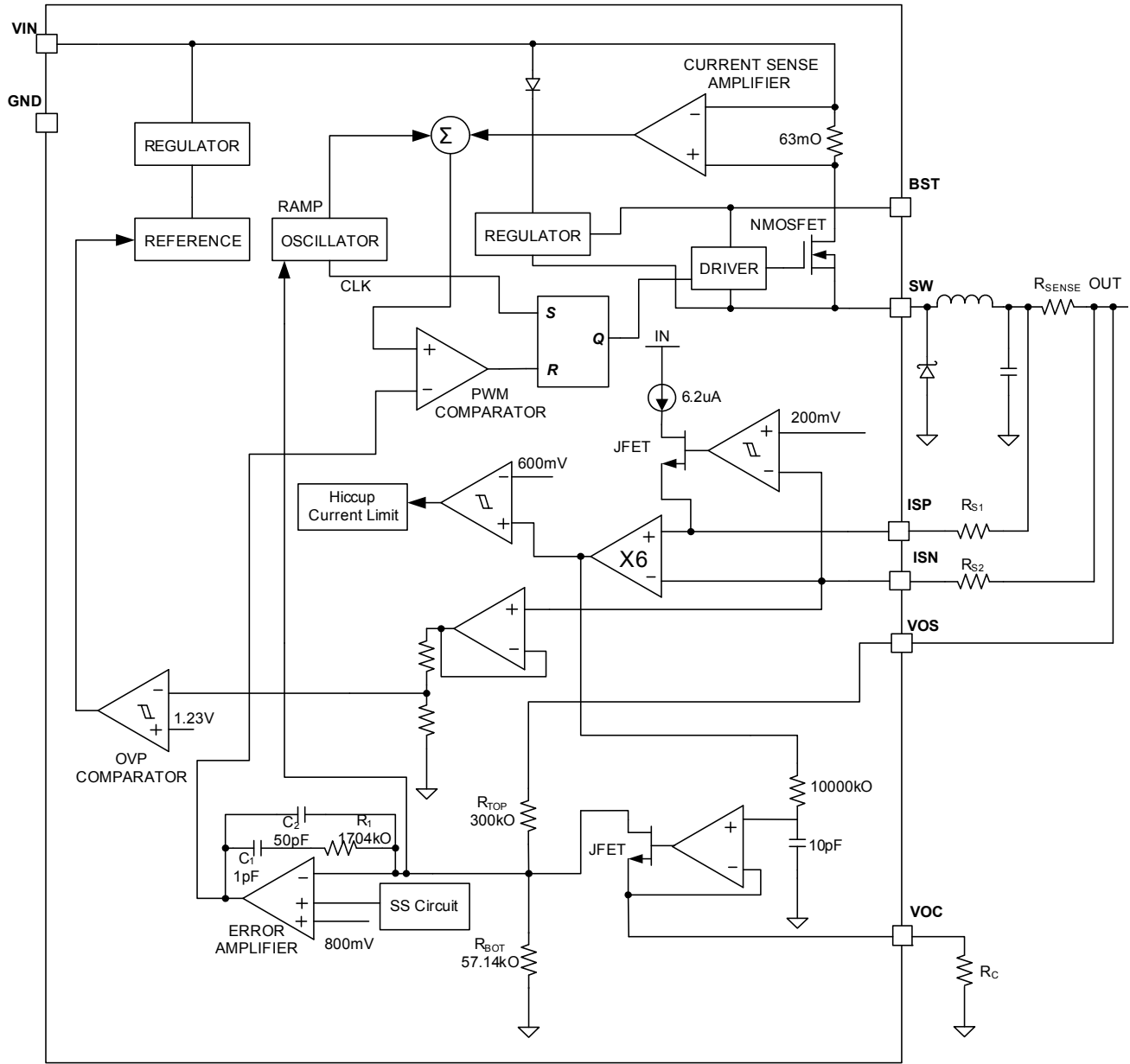
Figure 1—Function Block Diagram
