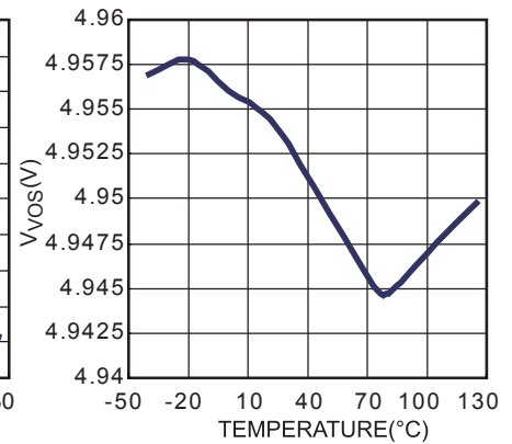
V VOS vs. Temperature
