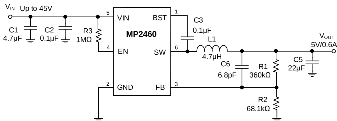
Figure 6: Typical Application Circuit (5V Output)
