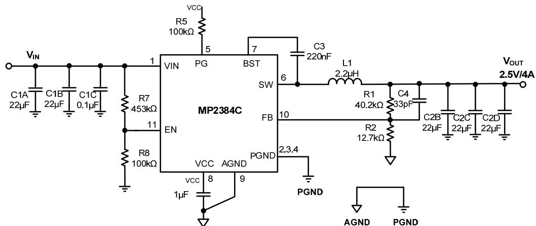
Figure 11: V_{IN} = 19V , V_{OUT} = 2.5V/4A
