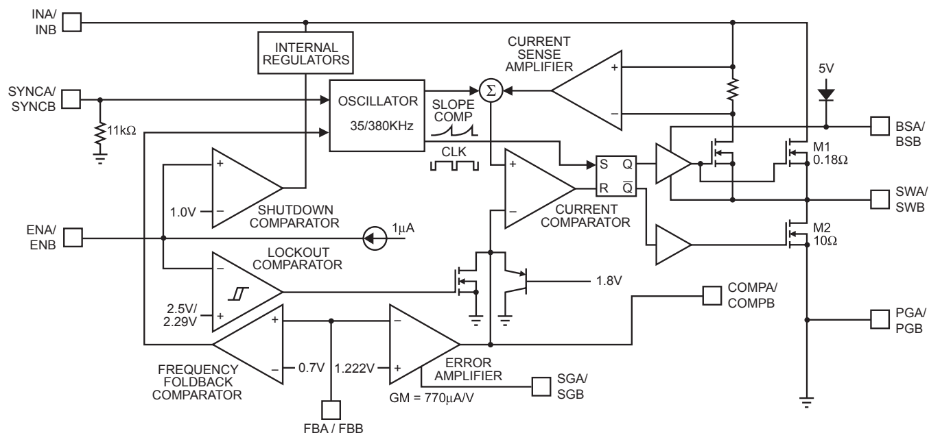
Figure 1—Functional Block Diagram (Diagram portrays ½ of the MP2362)
