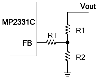
Figure 4: Feedback Network
