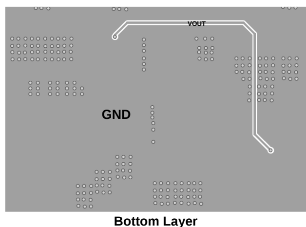
Figure 5: Recommended Layout
