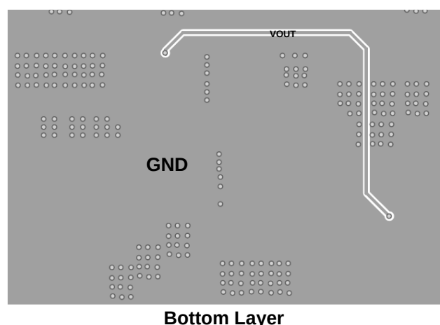
Figure 5: Recommended Layout
