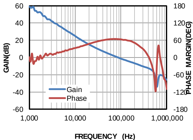
Bode Plot
