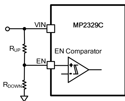
Figure 5: Adjustable UVLO
