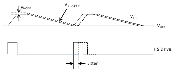
Figure 3: Jitter in Skip Mode
