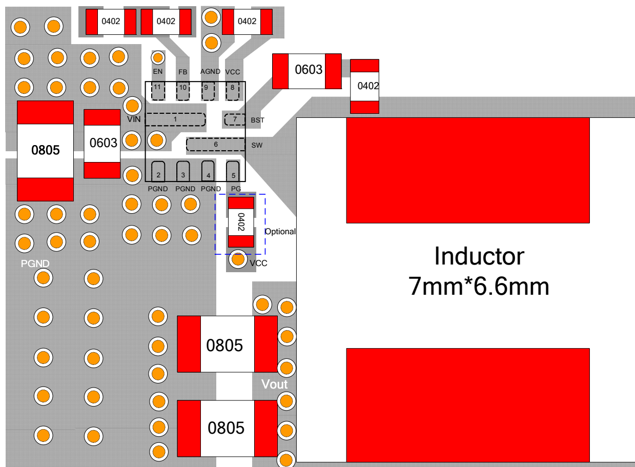
Figure 8: Recommended Layout
