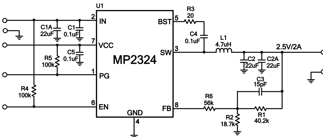
Figure 10: V_o=2.5V , I_o=2A
