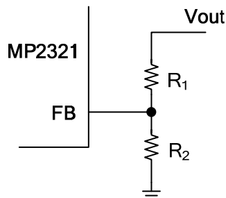
Figure 8: Feedback Network
