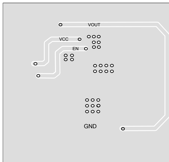
Figure 8: Sample Board Layout
