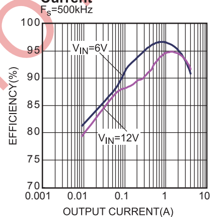
Efficiency vs. Output Current F_s = 500\text{kHz}
