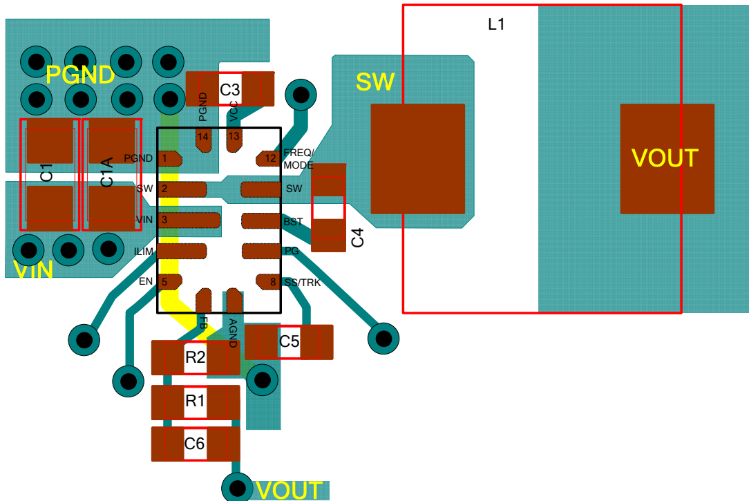
Figure 7: Recommended Layout
