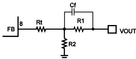
Figure 3: T-Type Network
