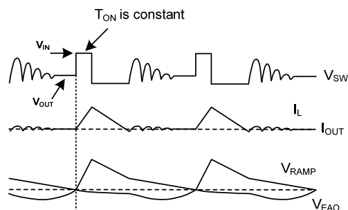
Figure 3: Light-Load Operation
