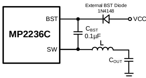
Figure 4: Optional External BST Diode to Enhance Efficiency
