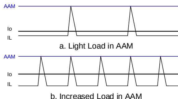
Figure 3: AAM Comparator Control t_{ON}
