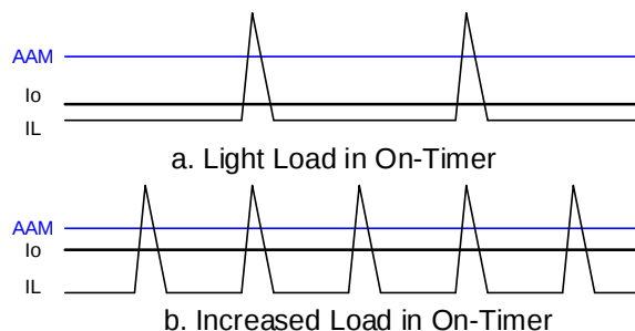
Figure 4: On-Timer Control t_{ON}
