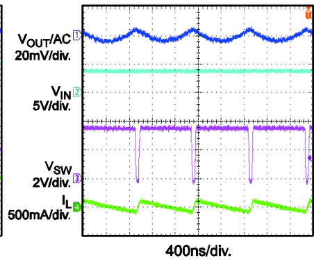
Steady State
