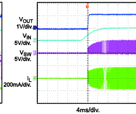
VIN Power-Up
