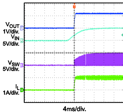
VIN Power-Up
