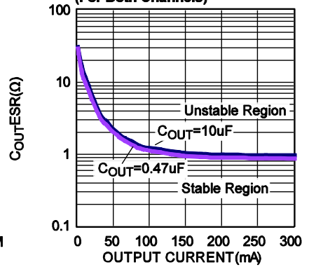
CO OUT ESR Stability vs. Output Current
