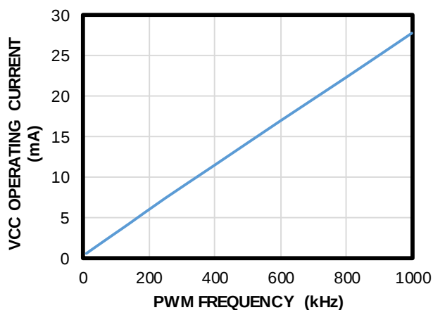
VCC Operating Current
