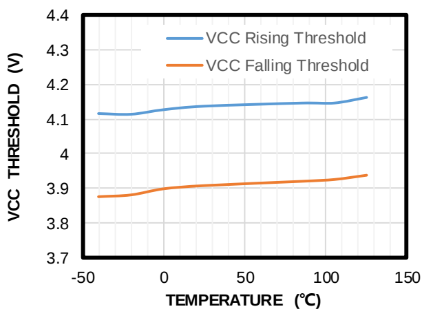
VCC Threshold vs. Temperature
