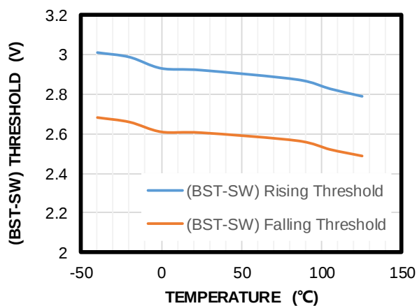
(BST-SW) Threshold vs. Temperature
