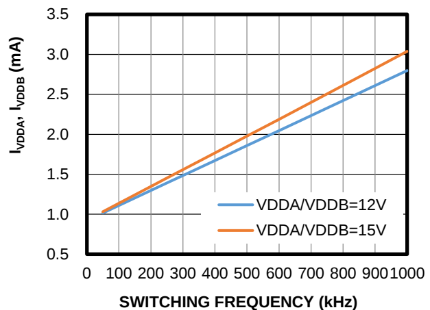
VDDA, VDDB Operating Current vs. f_{SW}
