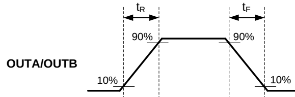
Figure 1: Output Rising and Falling Time
