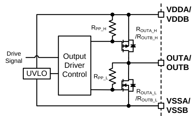
Figure 8: Output Stage
