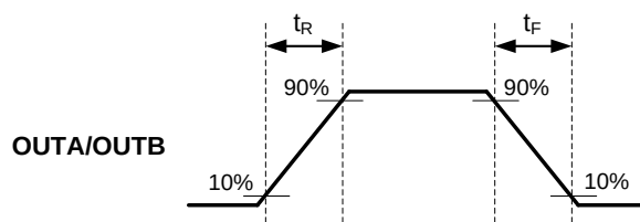
Figure 1: Output Rising and Falling Time
