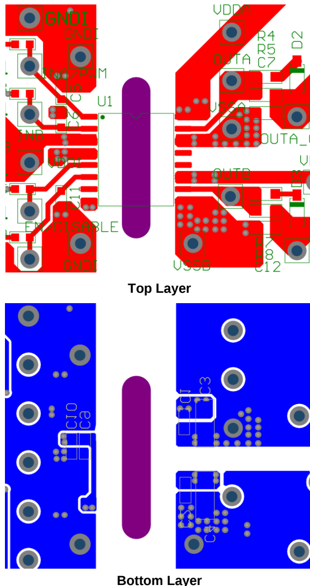
Figure 11: Recommended PCB Layout (20)
