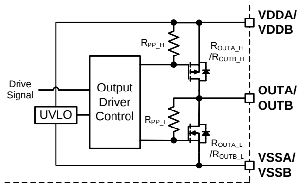
Figure 7: Output Stage
