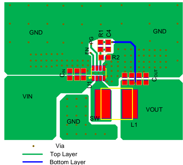
Figure 7: Recommended PCB Layout
