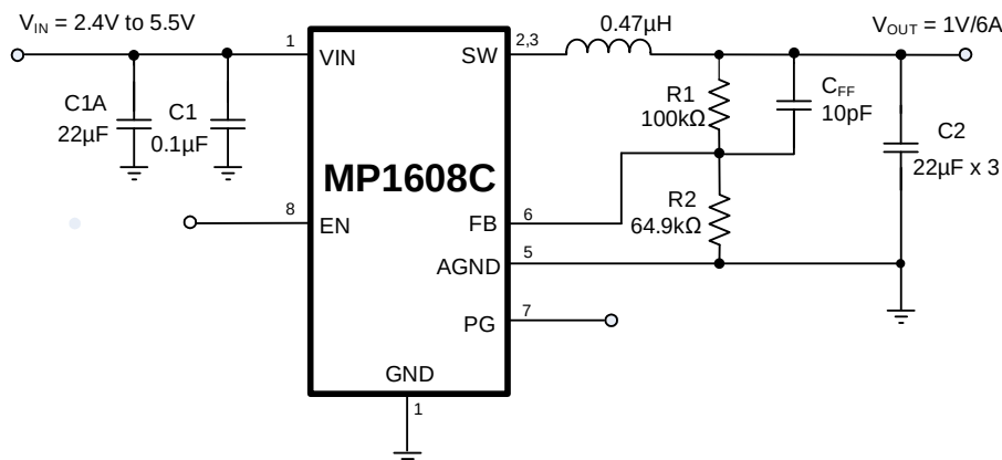
Figure 6: Typical Application Circuit ( V_{IN} = 2.4V to 5.5V , V_{OUT} = 1V/6A )
