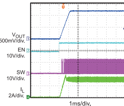
Start Up Through EN I_{OUT} = 3A
