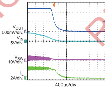
Shut Down Through VIN I_{OUT} = 2A
