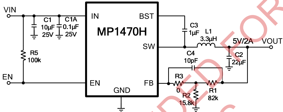
Figure 9: 12Vin, 5V/2A
