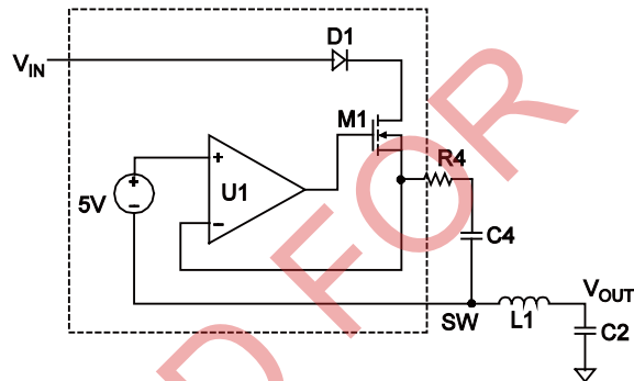
Figure 3: Internal Bootstrap Charger Start-Up and Shutdown Circuit
