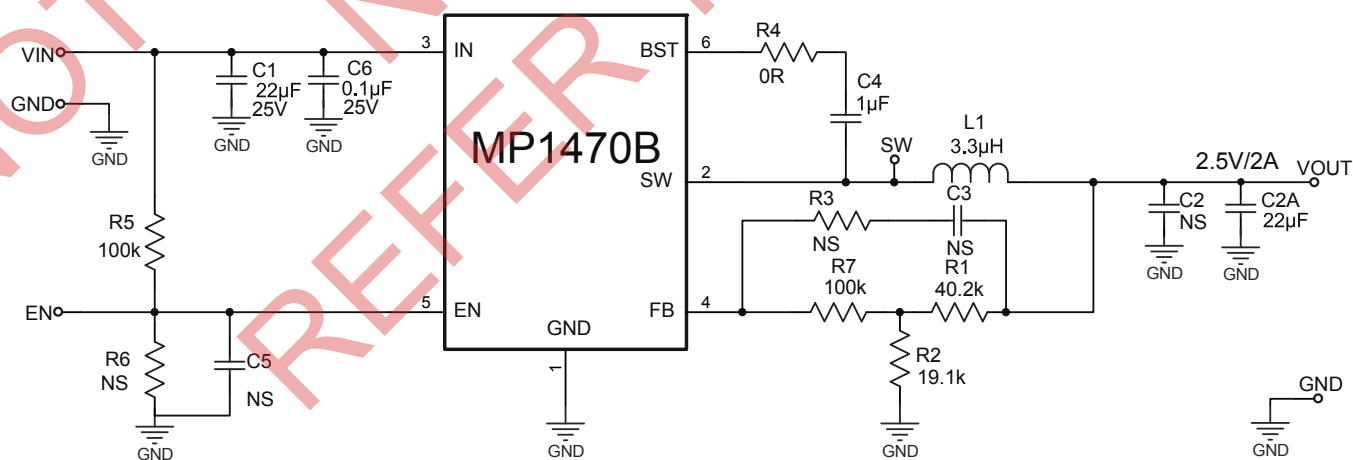
Figure 9: 12Vin, 2.5V/2A
