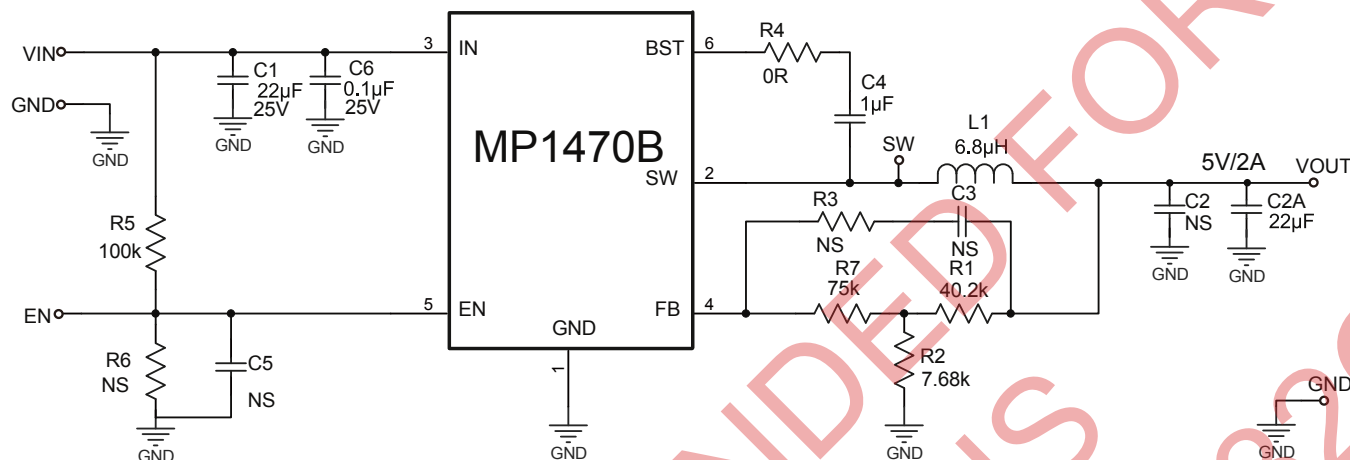
Figure 7: 12Vin, 5V/2A
