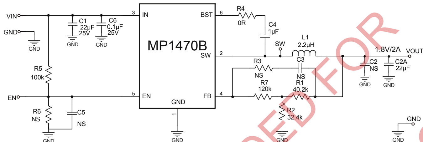
Figure 10: 12Vin, 1.8V/2A
