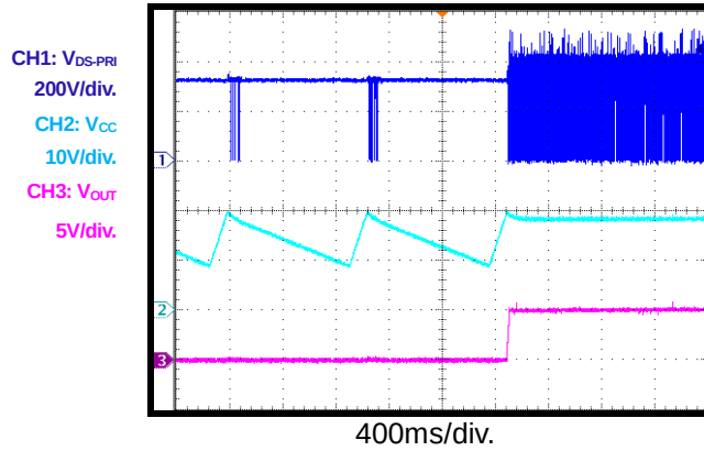
Short-Circuit Recovery
