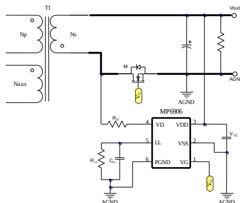
Figure 12: Synchronous Rectifier
