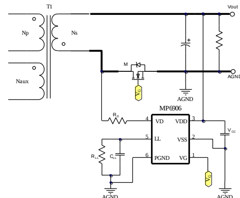
Figure 12: Synchronous Rectifier
