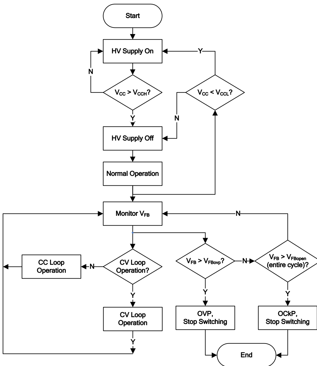
Figure 17: Flow Chart
