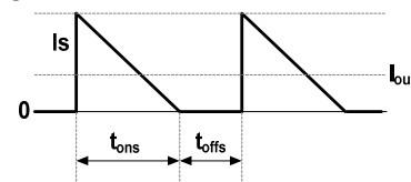
Figure 8: Secondary Current Waveform
