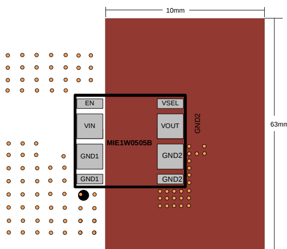
Mid-Layer 3
