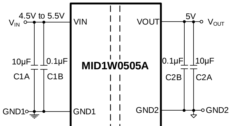
Figure 4: Application Circuit
