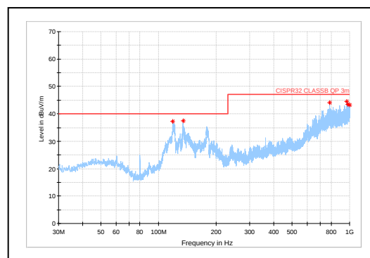
Radiated Emission 30MHz to 1GHz, CISPR32 Class B (8)
